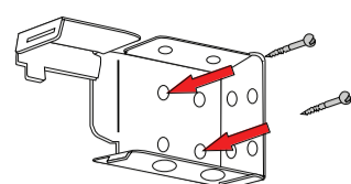
Side-Fixing: Where the bracket is fixed on to the side wall of a recess
